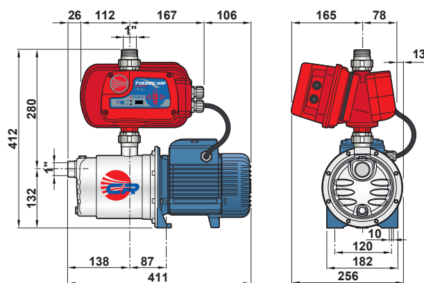
TS1-2CP 25/14 – TS1-2CP 25/16
